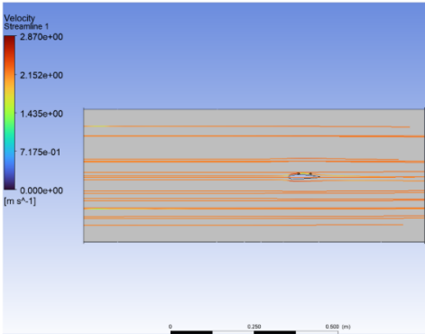
Airfoil Streamlines
