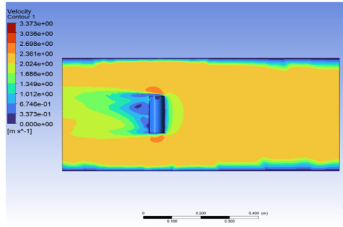
Cylinder Velocity
