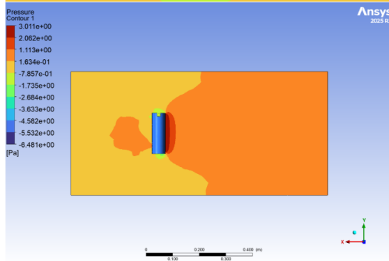
Cylinder Pressure
