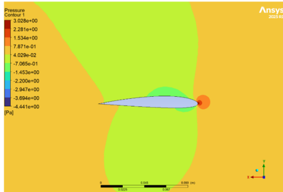
Airfoil Pressure
