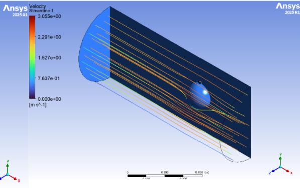
Sphere Streamlines
