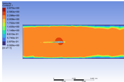
Airfoil Velocity
