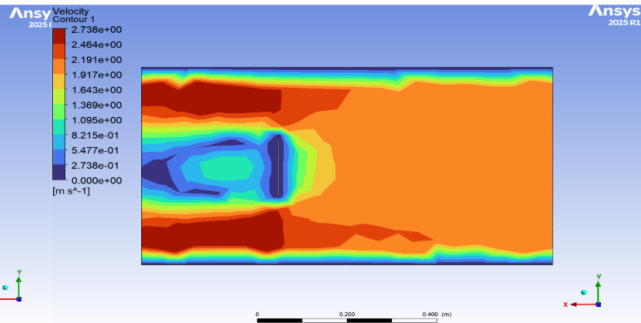
Sheet Velocity
