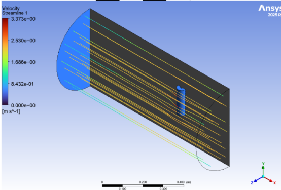
Cylinder Streamline
