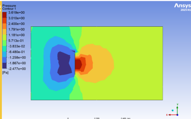
Sheet Pressure
