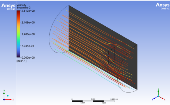
Sheet Streamlines
